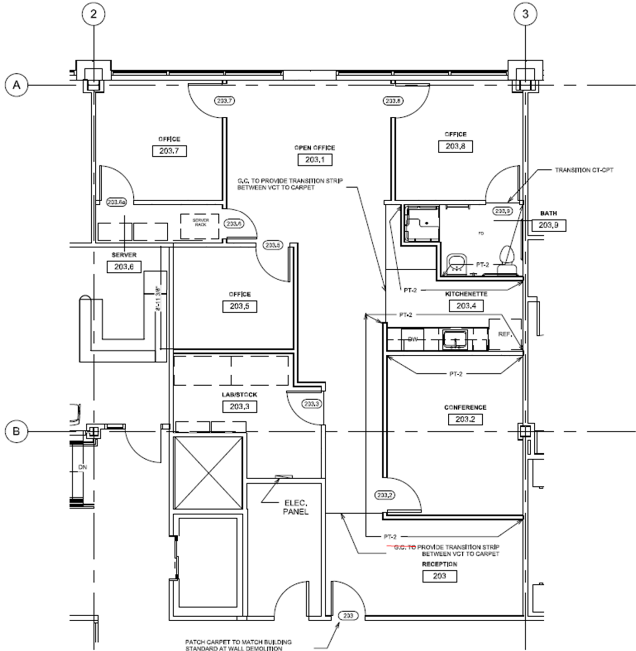
② Office Suite 203 Finish Plan 1/4" = 1'-0"
